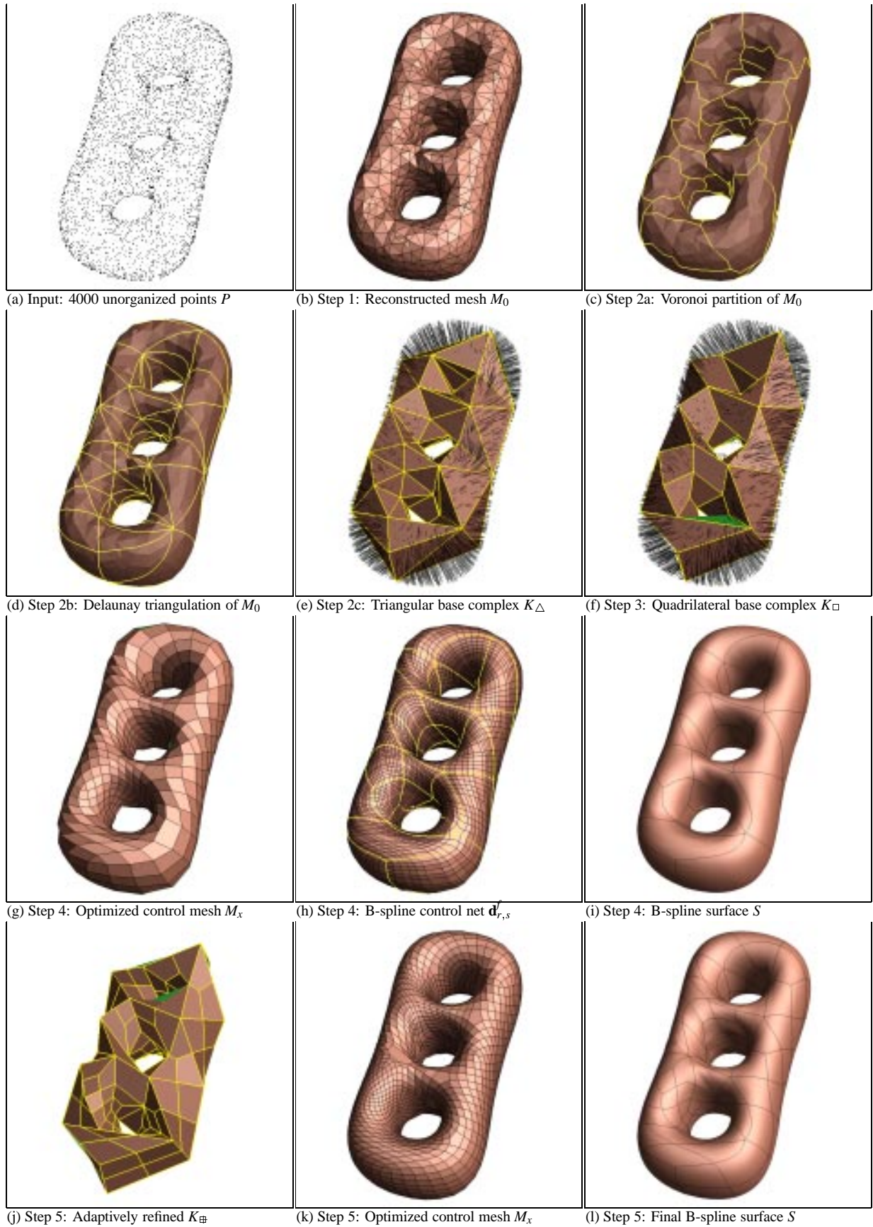
Figure 9: Illustration of the B-spline surface reconstruction procedure. From the points P in (a), the procedure automatically creates the G^1 B-spline surface in (l) which deviates from P by no more than 0.59% of the object's diameter.
